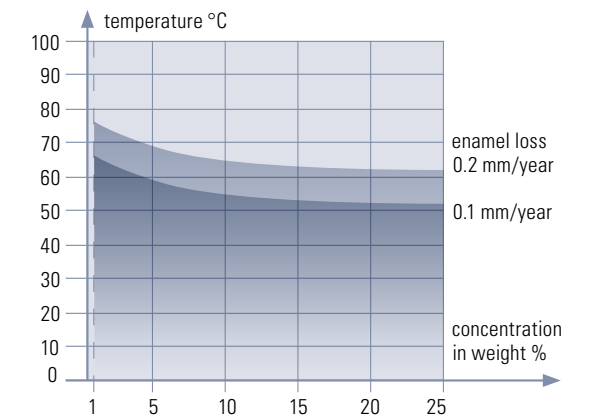
Corrosion velocity in HCL-aqueous solutions
