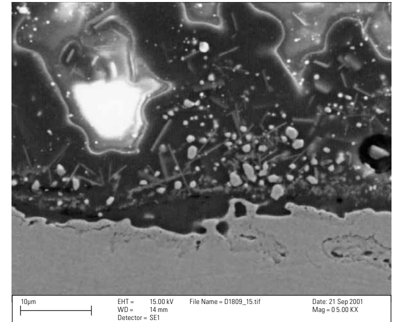
Fig. 2: Detail photograph of a compound layer enamel (in this case with grey cast iron (GGG) electron raster microscope photograph Fraunhofer-Institut ISC, Würzburg) in approx. 5,000-fold magnification. Clearly visible is the (micro) roughness of the surface (bright to the bottom) with back cuts. Following to the top is a thinner homogeneous appearing seam about 2 µm thick and the actual bonding layer afterwards clearly over 10 µm thick with different precipitations (ferrotitanium crystal in needle and pellet form) and inclusions.
