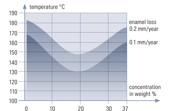
Corrosion velocity in HCL-aqueous solutions
