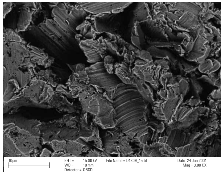
Fig. 3: Detail photograph of a corundum-blasted steel surface, approx. 3,000-fold magnification (raster electron microscope photograph Fraunhofer-Institut ISC, Würzburg). The surface as a result of the blasting operation is clearly split and eroded. This finish offers an ideal surface for building up the material compound in the subsequent enamelling process.
