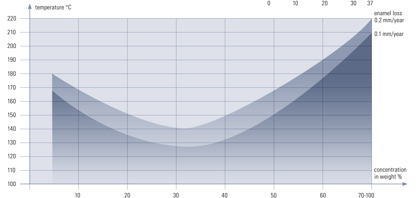
Corrosion velocity in H 2 SO 4 -aqueous solutions
